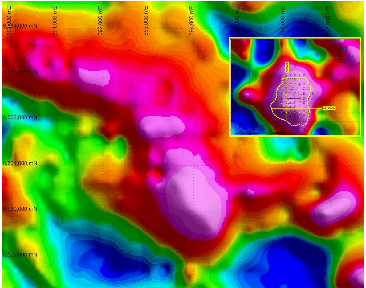
Figure 7: Lucas Hill Project - Residual Gravity Image with inset of Carapateena Residual Gravity Image at same scale.
