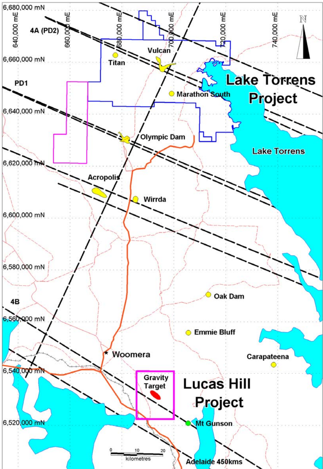
Figure 6: Tasman Lake Torrens and Lucas Hill Project Locations showing selected key historic tectonic lineaments, IOCGU deposits/prospects (yellow) and Lucas Hill gravity target.
